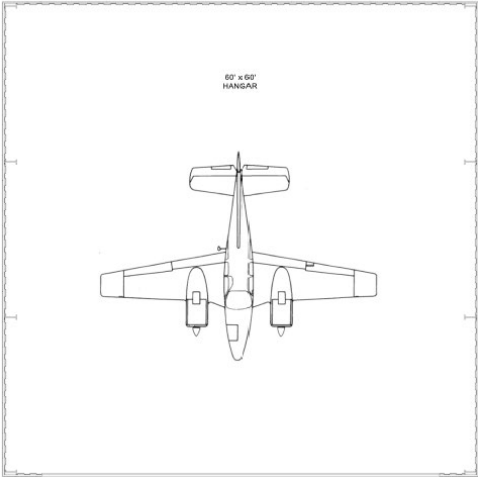
Large Hangar Floor Plan
